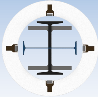
I & H Beam Max: 10 in.
